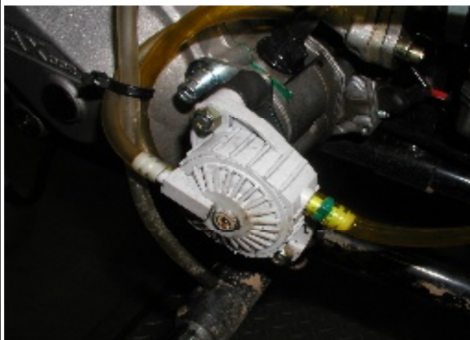
Foto of the frame with the section of the support for the fuel pump (fuel pump mounted)
