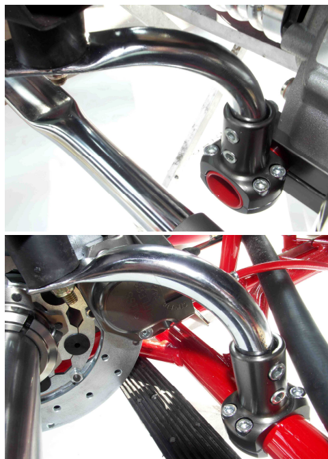
Photo from above of the frame with the section of the two supports for the exhaust system
