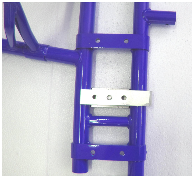
Foto from above of the frame with the section of the engine mount
