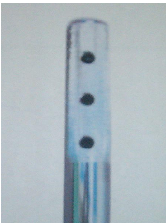
Photo from the steering column with the section with the knurling for the steering wheel hub (knurling according to DIN 82 - RAA1).
